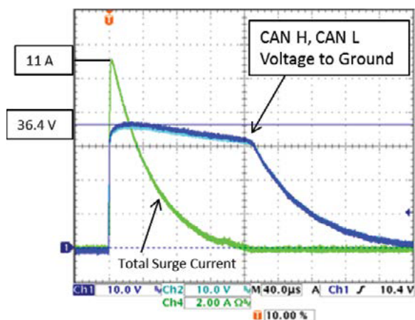
Figure 1 - CDSOT23-T24CAN Clamp Voltages for a +500 V Surge
